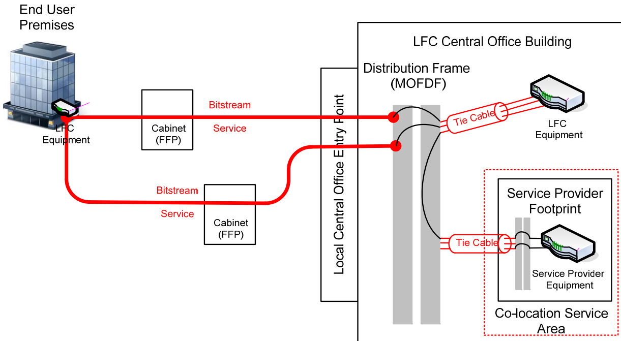
Single Central Office redundancy with separate diverse fibre and diverse access to End User Premises
